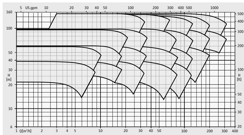
3000 rpm, 50 Hz: CN / CNF / CNK – single-stage series
