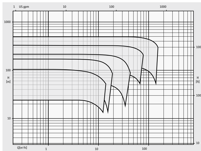
3000 rpm, 50 Hz: CAM – multi-stage series
